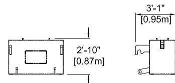
Carbody Counterweight 2 Pieces Weight: 10,000 lbs (4535kg)
