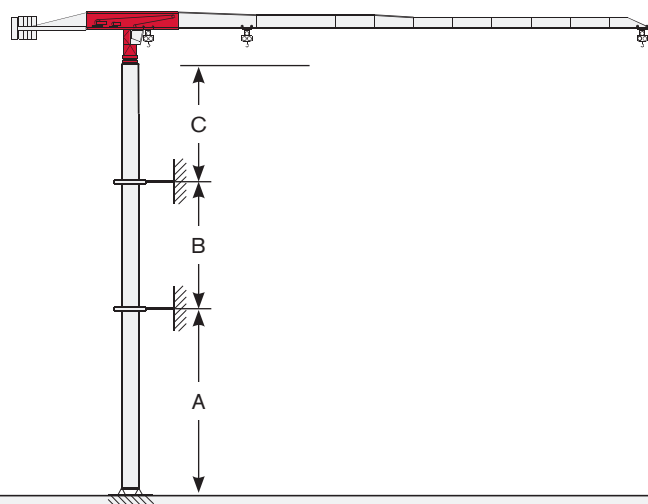
Tower: TS16
